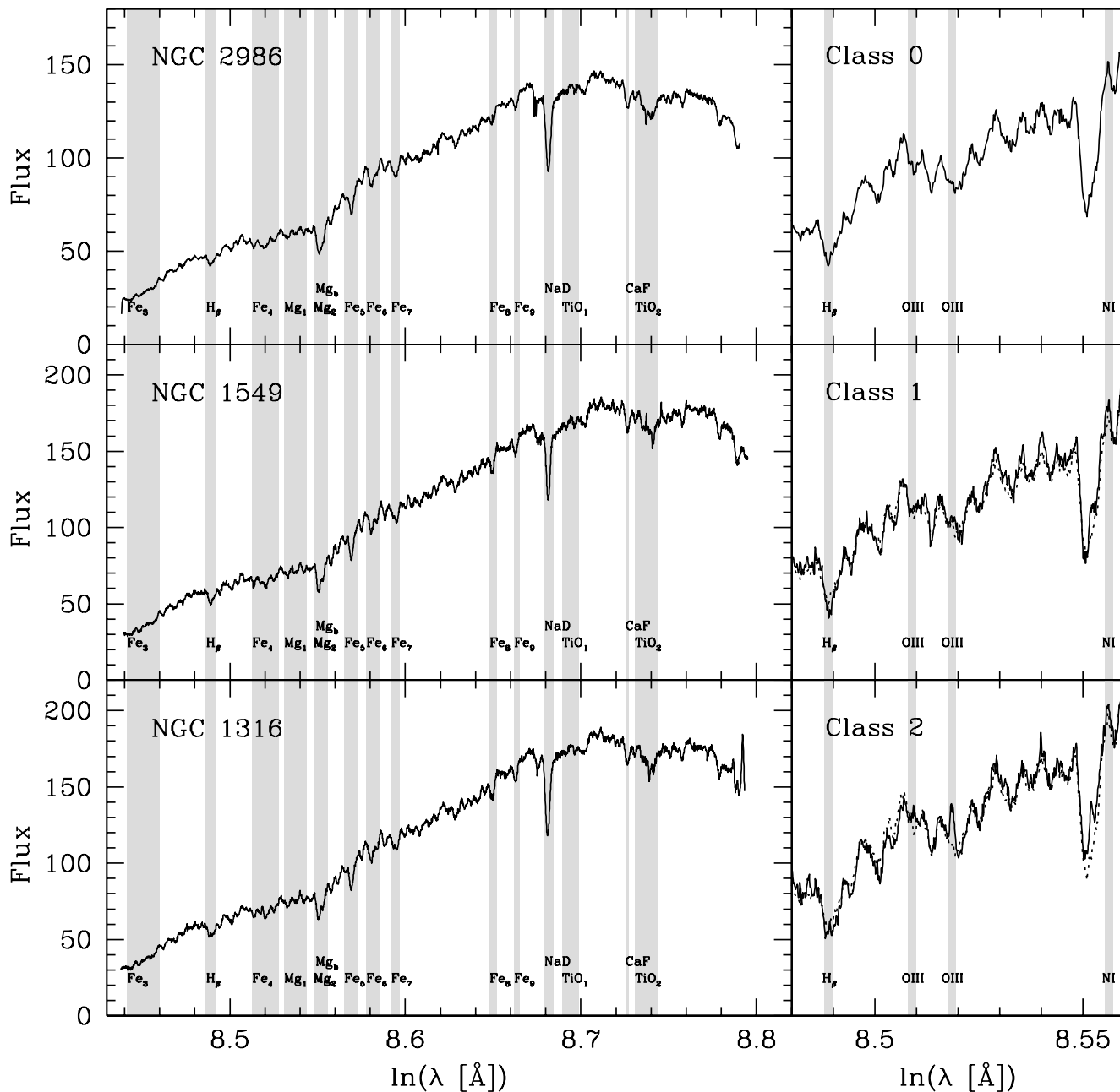
Fig. 8. Three examples of spectra with good signal-to-noise ratios plotted against the natural logarithm of the wavelength. Left panels: the full spectra transformed to zero redshift are shown. The flux is given in arbitrary units. Overlaid in light grey are the windows of the Lick/IDS indices measured in this work. Right panels: zoom of the spectra around the Fe5015 feature. In the upper left corner the emission class is indicated. Overlaid in light gray are the positions of emission lines. The dotted spectrum in the lower two panels is of NGC 2986, rescaled to match the spectra of NGC 1549 and NGC 1316.
