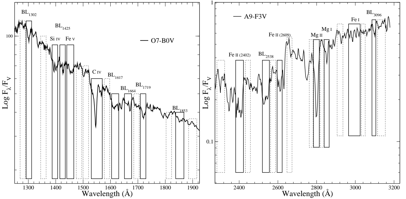
Fig. 2. Visualisation of index bandpasses on representative stellar spectra. The left-hand panel shows the far-UV indices with the central bandpasses highlighted by solid boxes and the blue and red continuum bandpasses marked by dotted boxes. The right panel shows, in the same way, the mid-UV indices. The bandpasses for the Mg_{\text{wide}} index are not depicted in order to avoid crowding.
