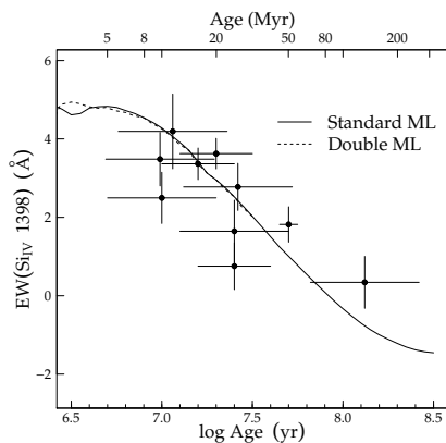
Fig. 17. Comparison between models adopting Geneva tracks with a standard (solid line) and twice the standard (dashed line) mass-loss rate for massive stars ( \gtrsim 15M_{\odot} ). No effect is appreciable.
