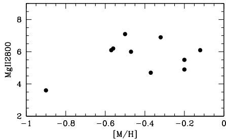
Fig. 13. The \text{Mg II } 2800 index of the LMC GCs as function of the metallicity as determined in the literature (see Table D.1 in the Appendix)..
