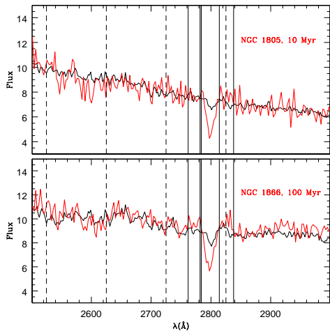
Fig. 11. Zoom of the spectral region containing the \text{Mg II } 2800 index. The observed spectra of two LMC clusters from the Cassatella et al. sample are shown in red, with overlaid template spectra from BC03 based on the Fanelli et al. library (black) at the age of the observed clusters (labeled in the panels). Vertical solid lines show the line and continua windows defining the \text{Mg II } 2800 index (cf. Table 1); dashed lines refer to the \text{Mg}_{UV} of Daddi et al. (2005).
