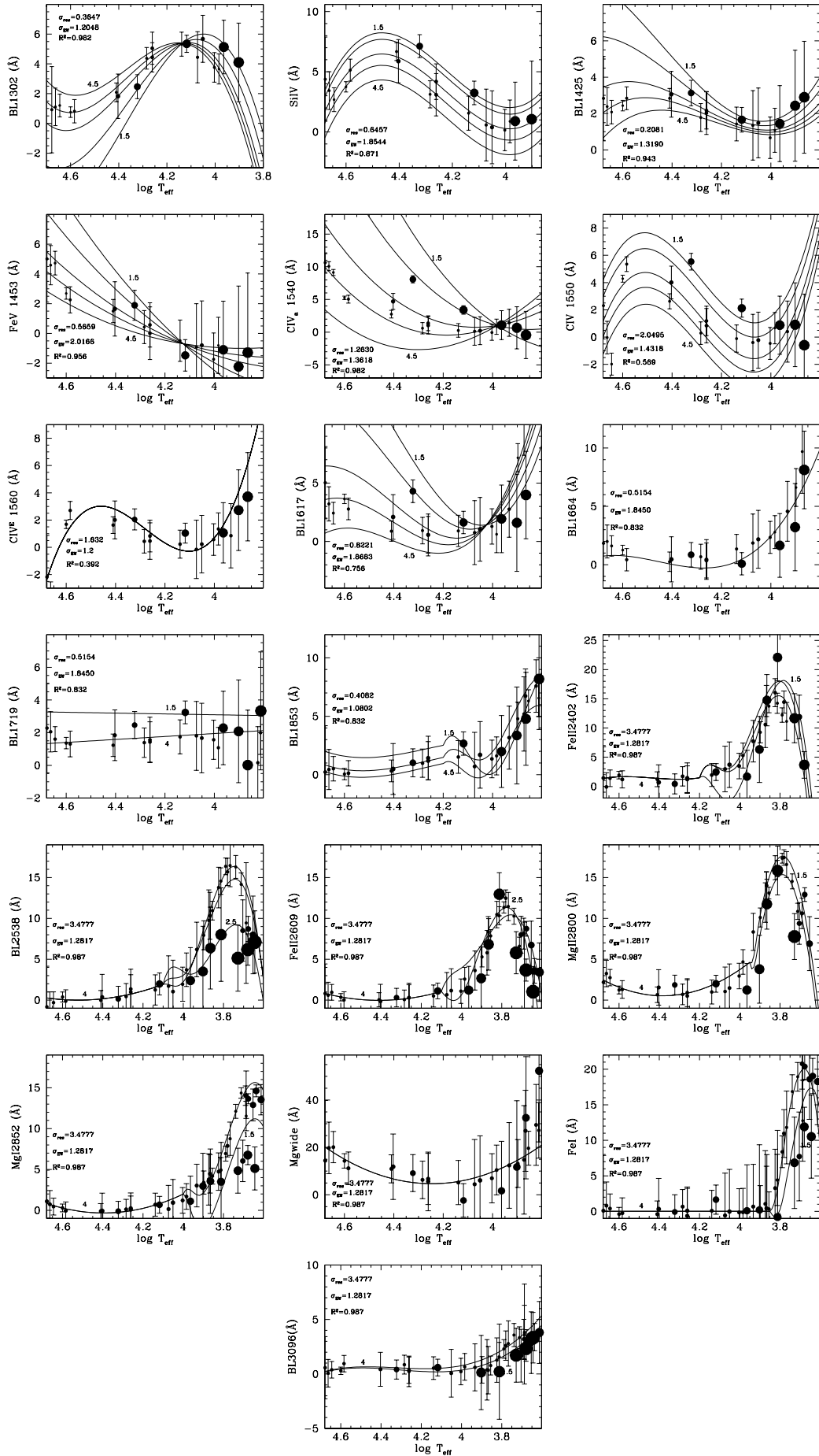
Fig. 5. Fitting functions. Stellar EWs are shown as functions of the effective temperature. The surface gravity is encoded in the symbol size (large circles for giants, small circles for dwarfs), using a linear function with a slope of 2.6 and a zero-point of 0.8. FFs for various gravities (see labels) are plotted. The standard deviation of the residuals ( \sigma_{\text{res}} ) and the mean equivalent width error \overline{\sigma_W} of all the groups included the fit are also shown.
