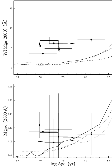
Fig. 12. Comparison between the \text{Mg II } 2800 from Fanelli et al. and the \text{Mg}_{UV} index defined in Daddi et al. (2005). In both panels, solar and half-solar metallicity models (solid and dashed lines, respectively) are plotted together with the GCs data. Also plotted are the indices as derived from Bruzual & Charlot (2003) solar metallicity models (dotted line), which use the same spectral library we use in the UV and give very similar results to ours.
