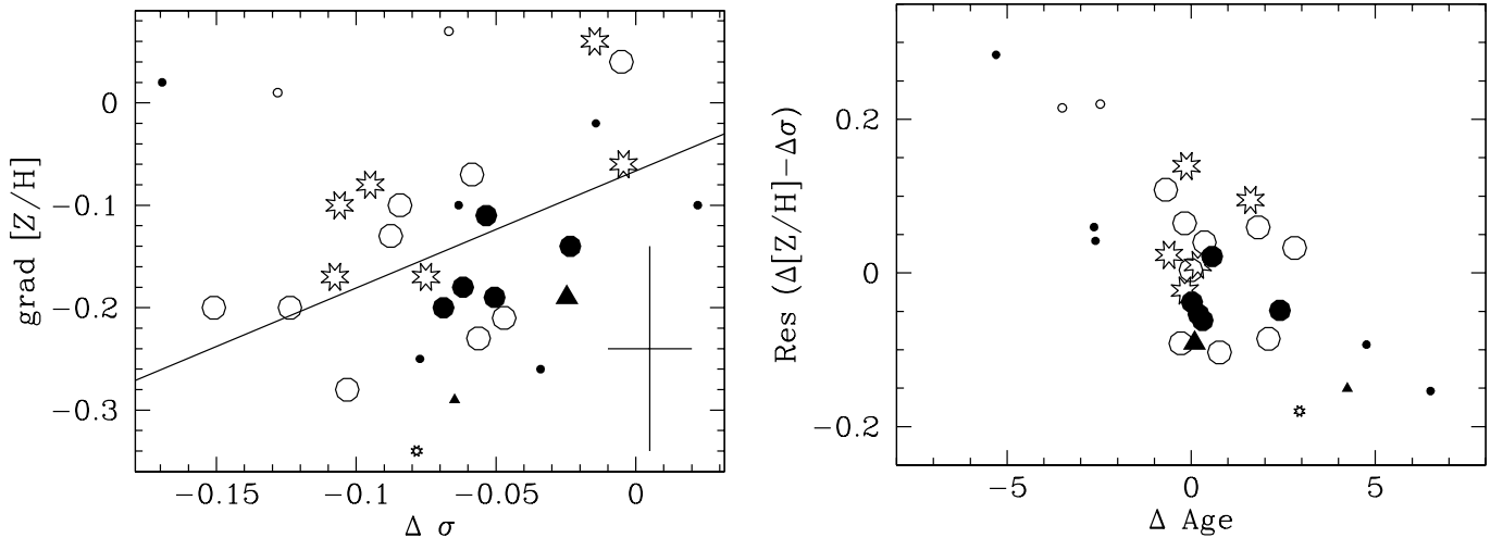
Fig. 8. Left panel: metallicity gradient as a function of the logarithmic gradient in velocity dispersion. Symbols as in Fig. 1. Galaxies outside one \sigma about the mean of the age gradients' distribution (see Fig. 7) are plotted with smaller symbols. The typical error is given in the lower right-hand corner. Right panel: residuals from the correlation shown in the left panel by the solid line as a function of the age gradient.
